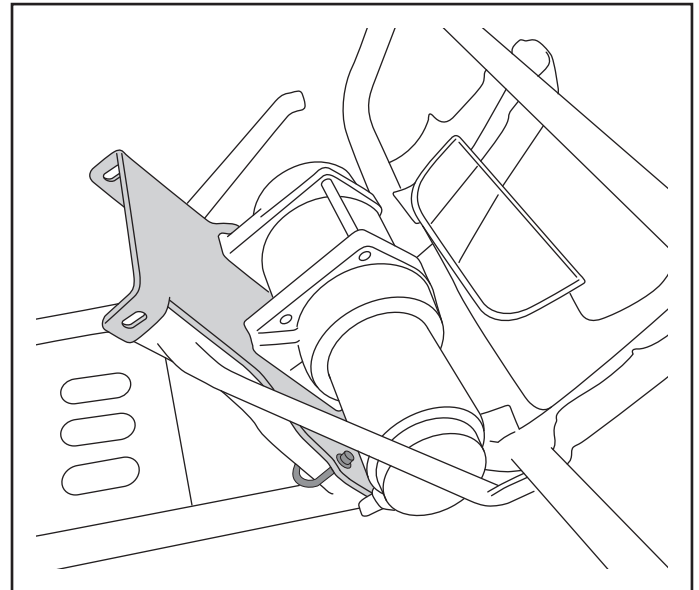
Figure 8. Installed Position
