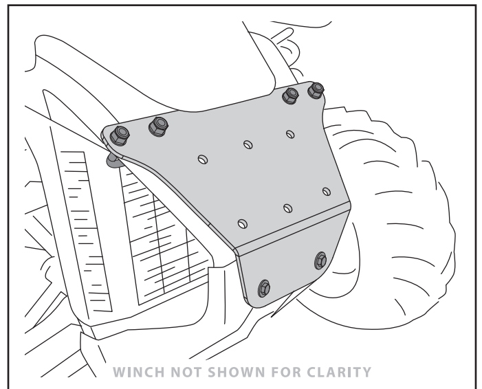
Figure 3. Installed position
