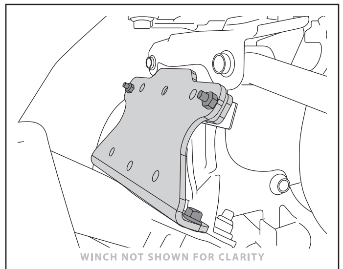
Figure 5. Installed position
