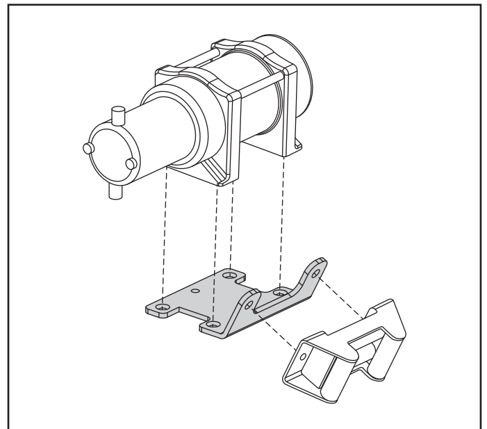
Figure 5. Standard winch configuration
