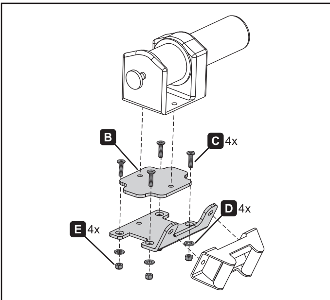
Figure 4. 2-hole winch configuration
