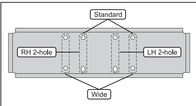
Figure 4. Winch hole configurations
