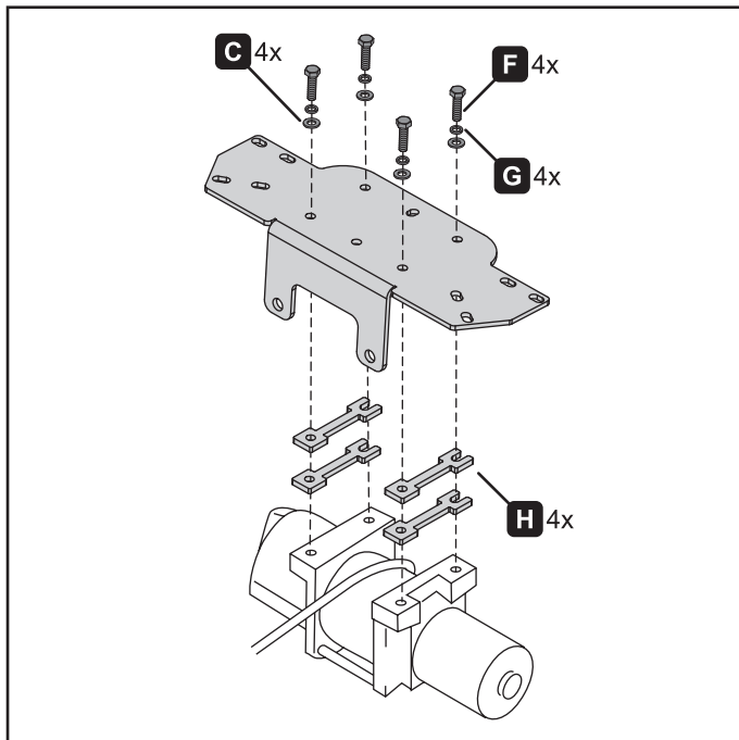
Figure 2. Four spacer configuration
