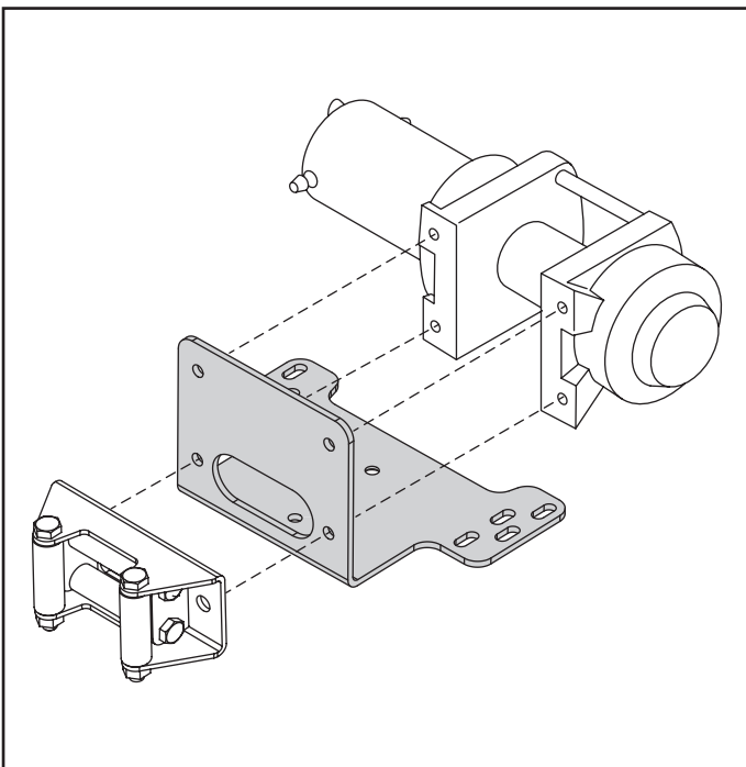
Figure 4. Standard winch configuration
