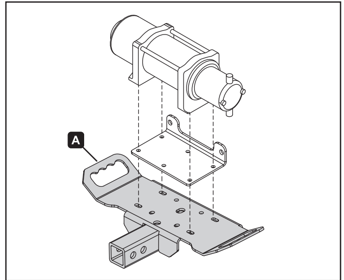
Figure 1. Wide winch install
