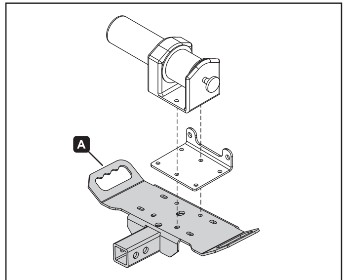
Figure 3. 2-hole winch install
