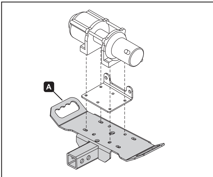
Figure 2. Standard winch install
