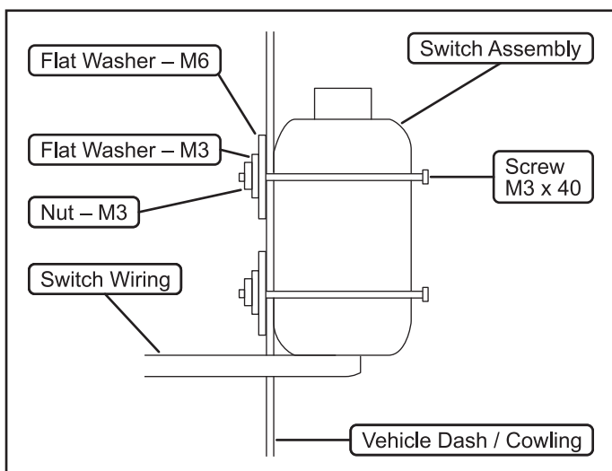
Figure 4. Optional switch mount instructions
