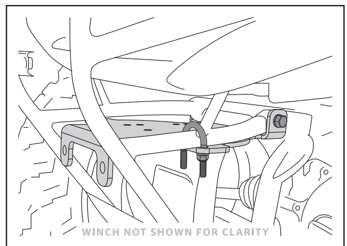
Figure 3. Installed position
