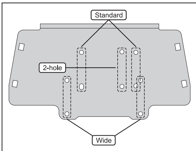
Figure 4. Winch hole configurations
