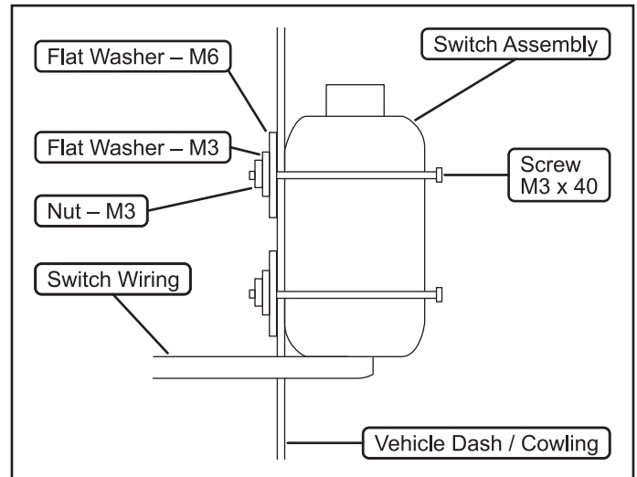
Figure 11. Optional switch mount instructions
