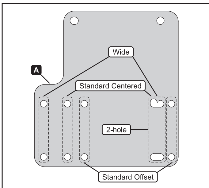
Figure 4. Winch hole configurations
