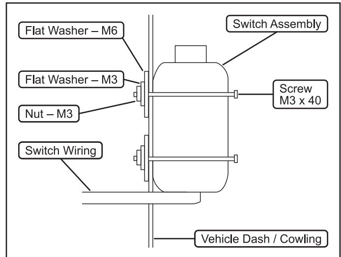
Figure 5. Optional switch mount instructions
