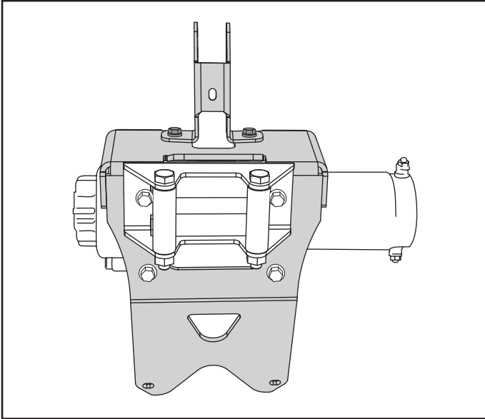
Figure 10. Installed position
