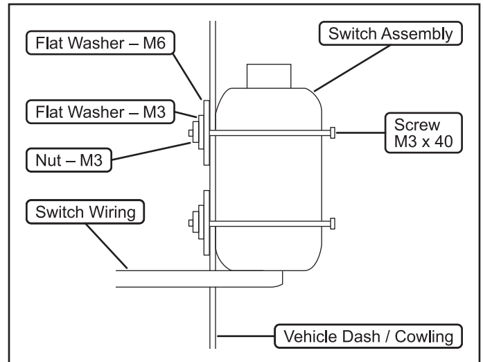
Figure 7. Optional switch mount instructions
