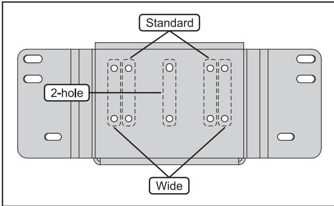
Figure 1. Winch hole configurations
