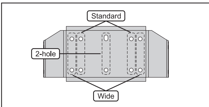
Figure 5. Winch hole configurations
