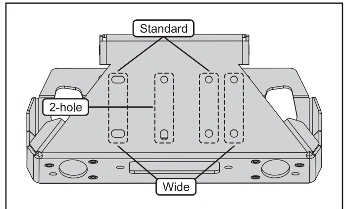
Figure 6. Winch hole configurations
