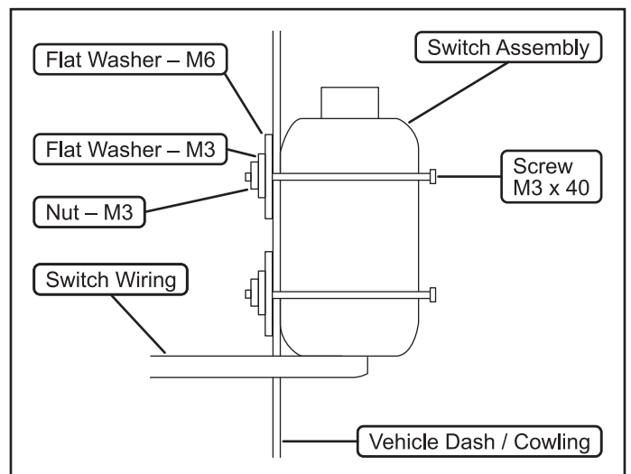
Figure 10. Optional switch mount instructions
