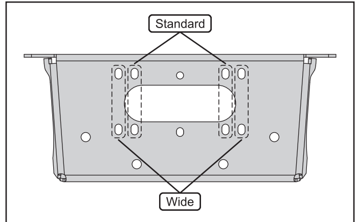
Figure 6. Winch hole configurations
