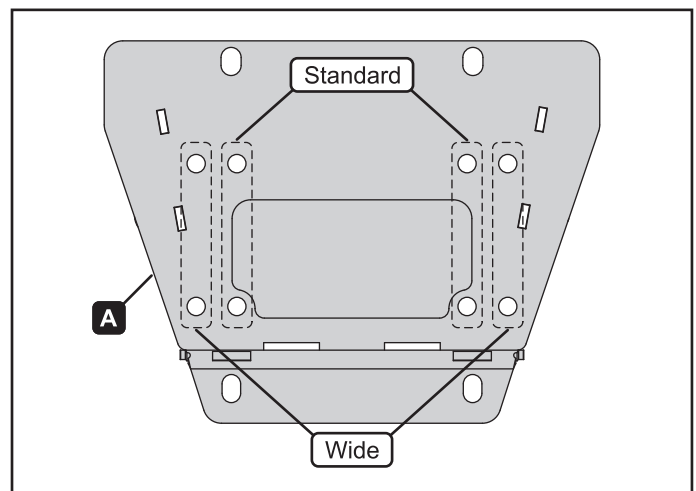
Figure 3. Winch hole configurations
