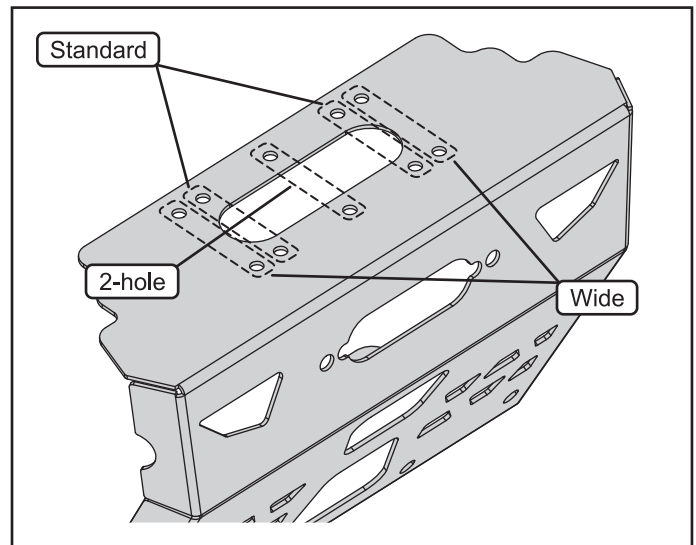
Figure 9. Winch bolt patterns
