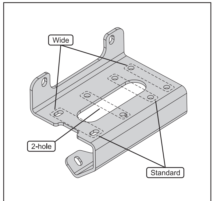
Figure 5. Winch hole configurations
