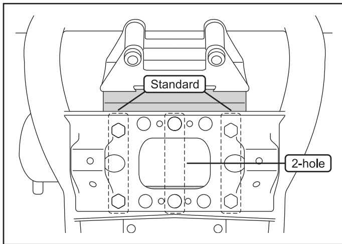
Figure 8. Winch hole configurations
