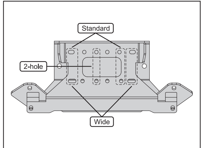
Figure 8. Top view winch hole configurations
