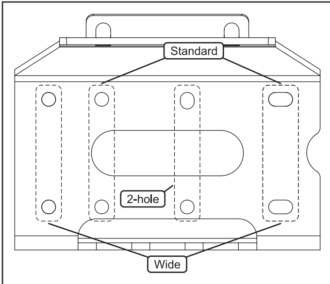
Figure 6. Winch hole configurations
