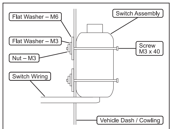
Figure 9. Optional switch mount instructions
