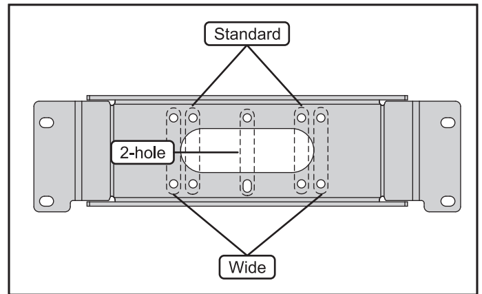
Figure 3. Winch hole configurations
