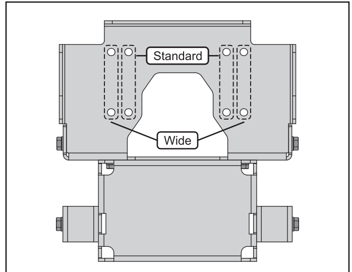
Figure 6. Winch hole configurations
