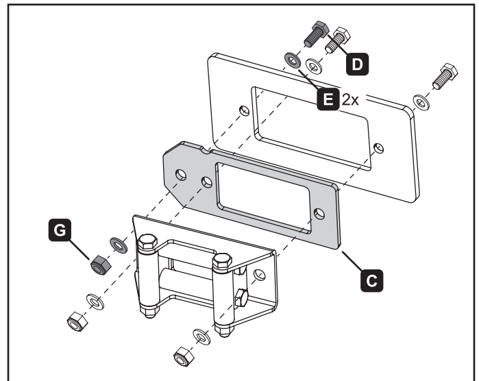
Figure 8. Bumper mount standard fairlead configuration
