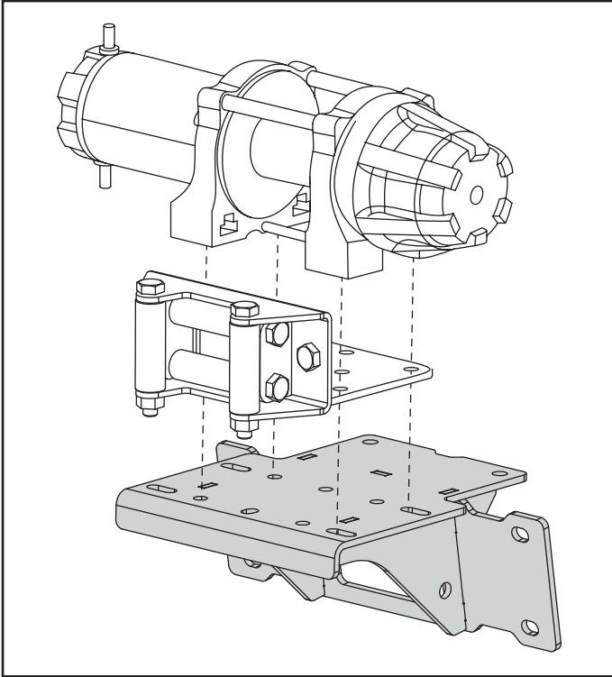
Figure 6. Without bumper mount fairlead configuration
