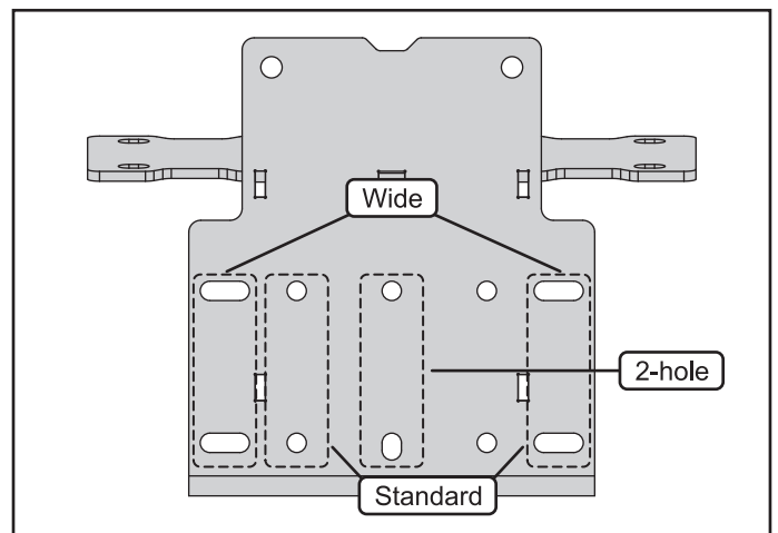
Figure 5. Winch hole configurations
