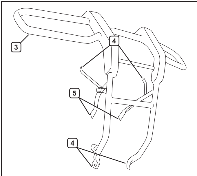
Figure 2. Lower front bumper bolts
