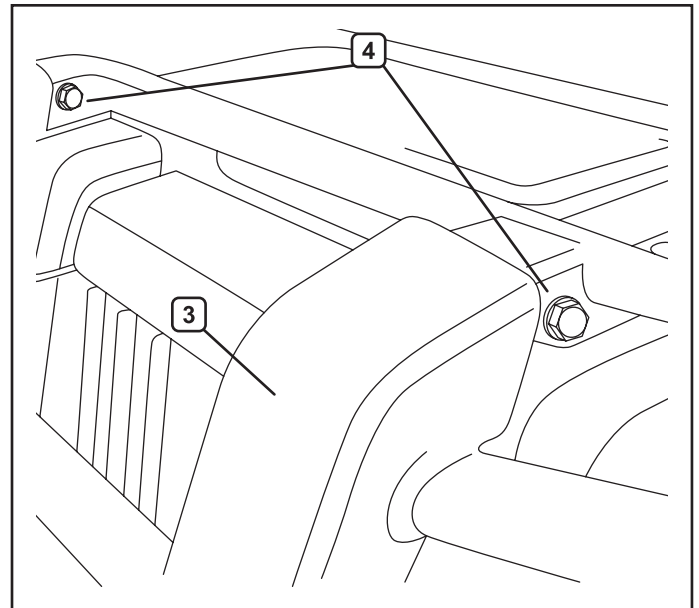
Figure 3. Upper front bumper bolts
