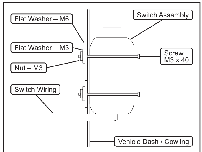
Figure 3. Optional switch mount instructions
