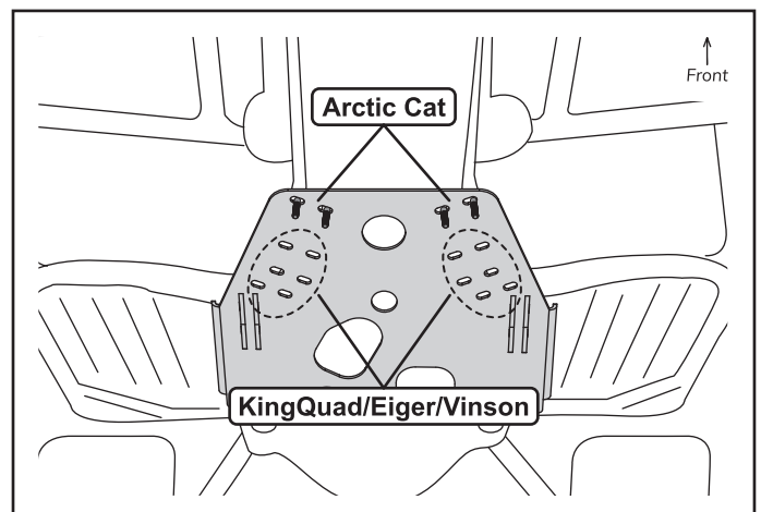
Figure 4. U-bolt position
